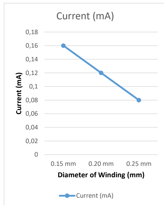
Pict. 8 Graphs of variation of circumferential diameter data with the resulting voltage
