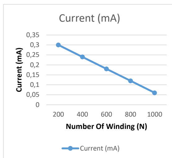
Pict. 5 Graph of the data variations of the number of winding with the current
