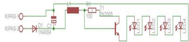
Pict. 2 Schematic Design
